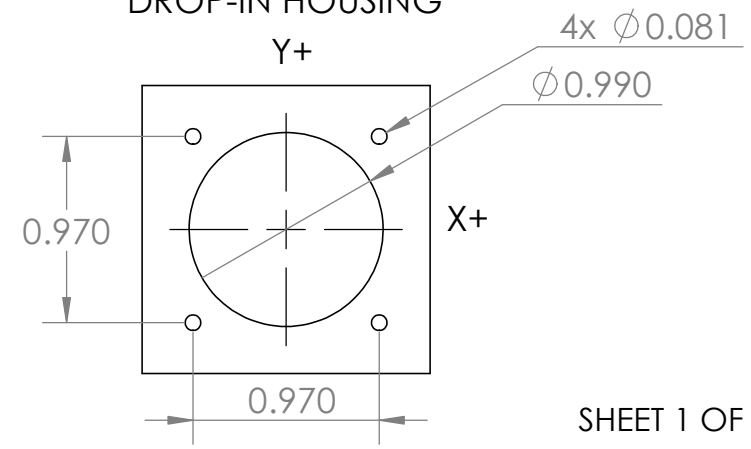
PANEL CUTOUT DIMENSIONS, DROP-IN HOUSING
