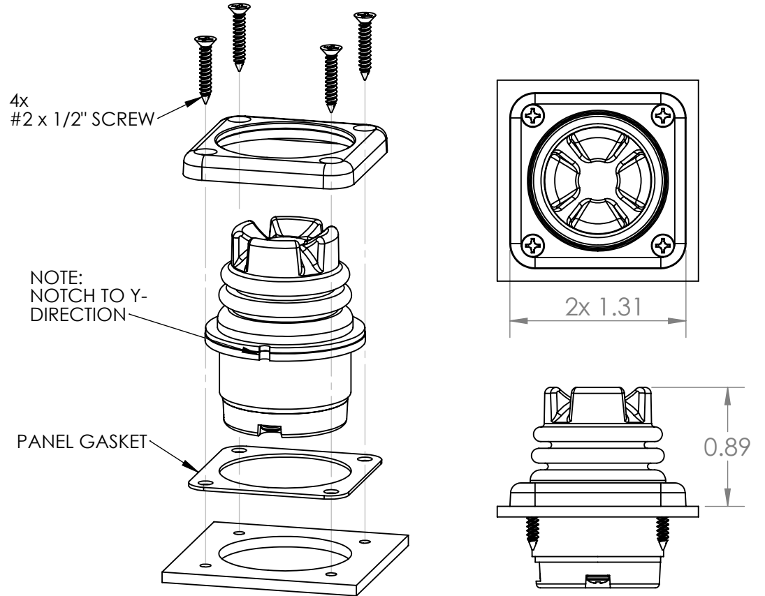
PANEL CUTOUT DIMENSIONS, DROP-IN HOUSING
